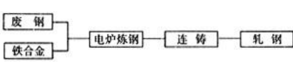
图2 电炉炼钢流程(EAF)普钢 CO 2 排放边界
